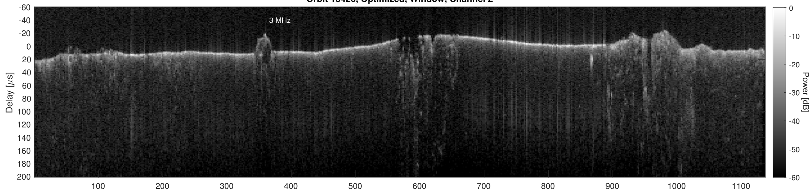
Orbit 13426, Cluttergram
