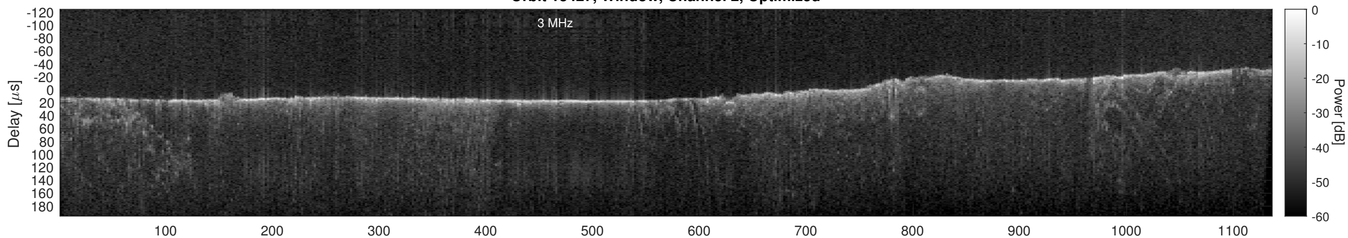
Orbit 13427, Cluttergram
