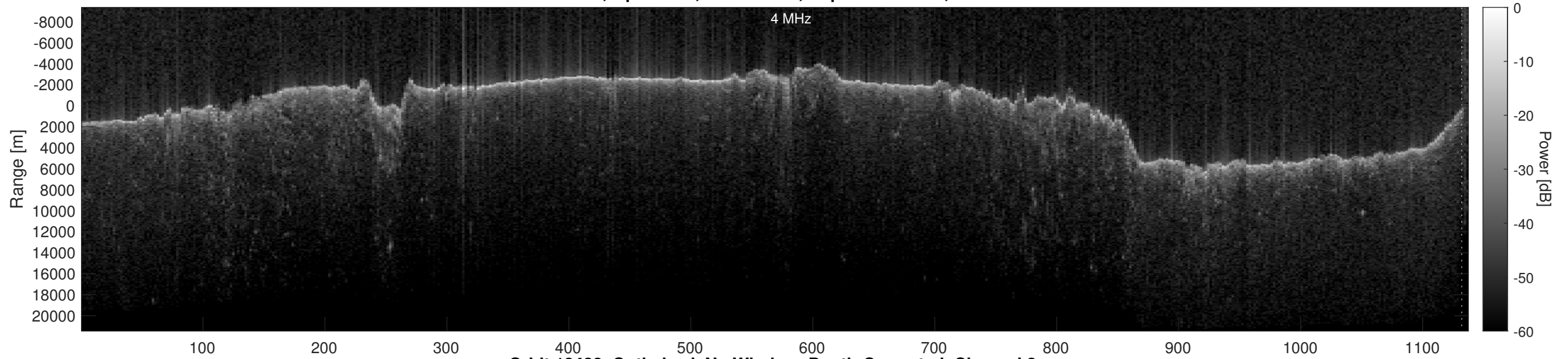
Orbit 13428, Optimized, No Window, Depth-Corrected, Channel 2
