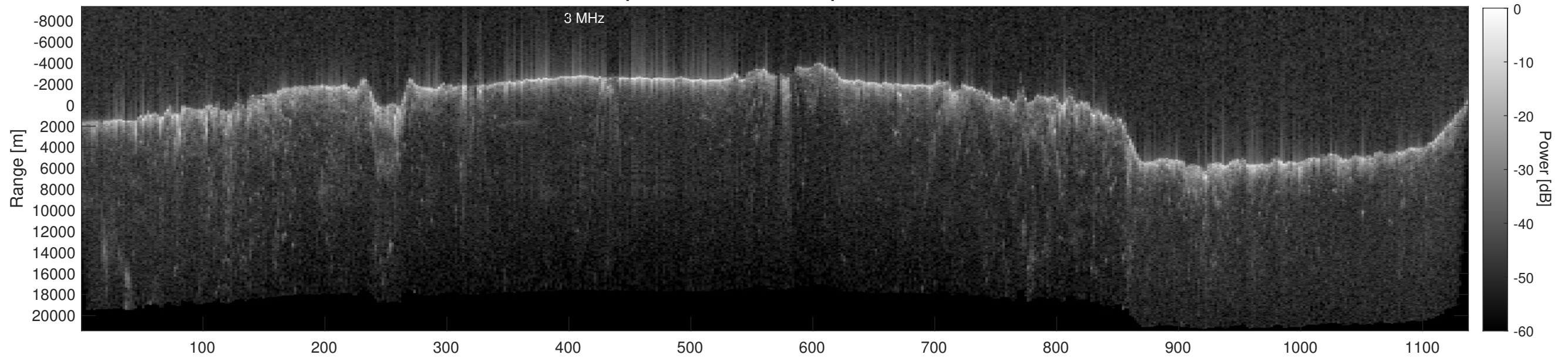
Orbit 13428, Depth-Corrected Cluttergram
