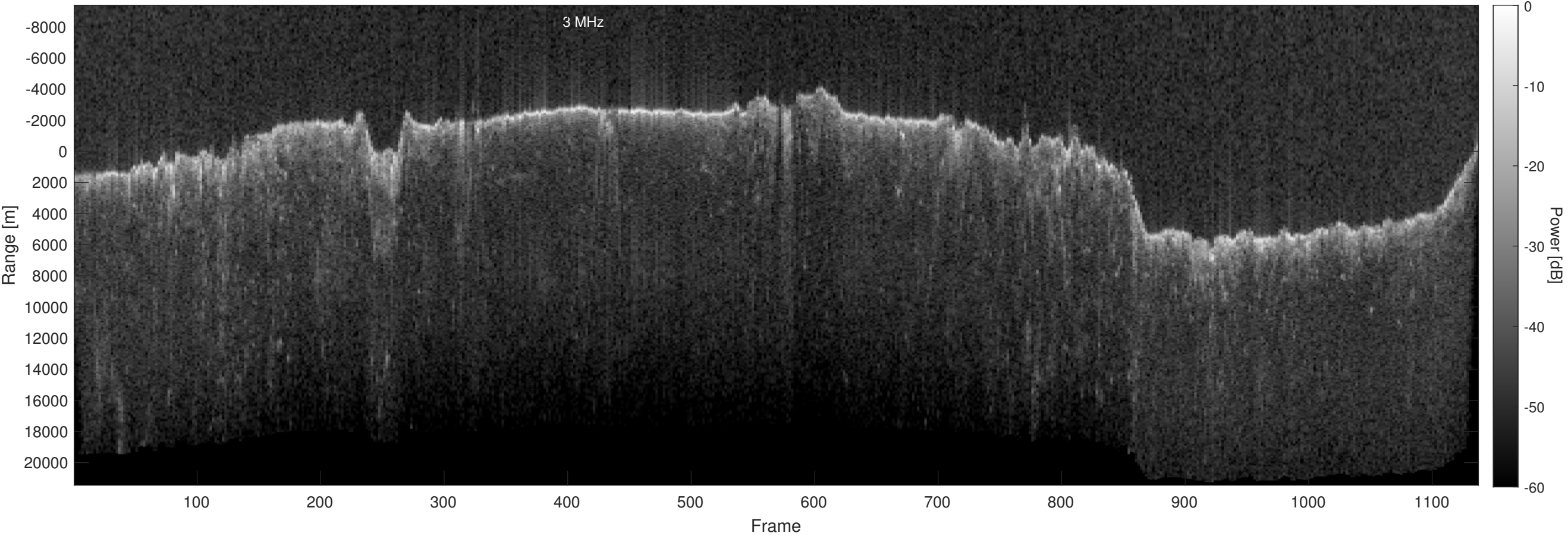
Orbit 13428, Optimized, Window, Depth-Corrected, Channel 2
