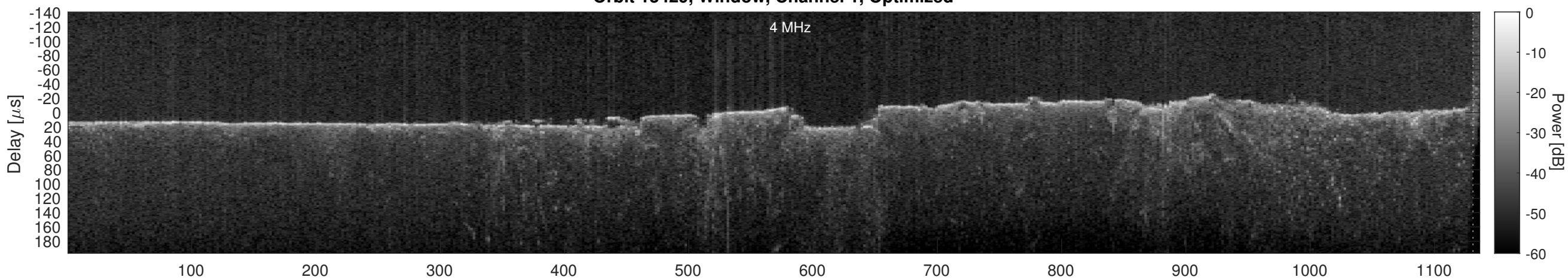
Orbit 13429, Cluttergram
