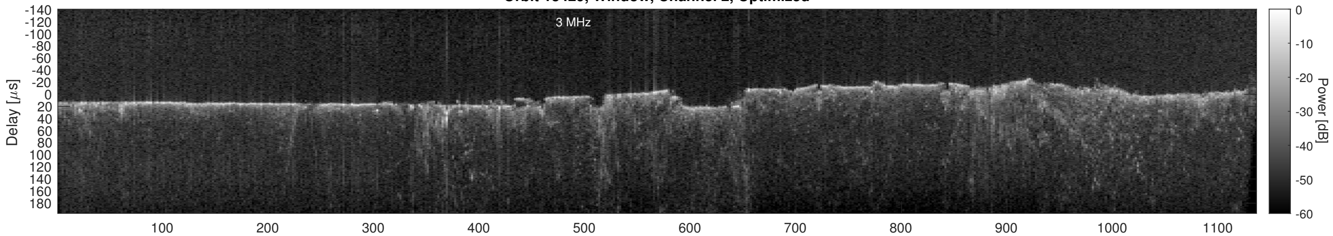
Orbit 13429, Cluttergram
