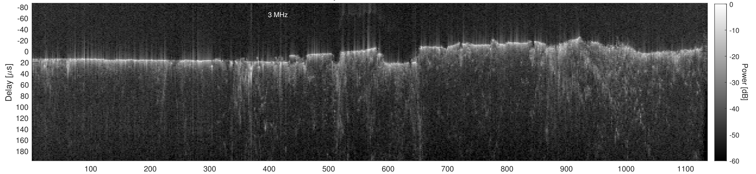
Orbit 13429, Cluttergram
