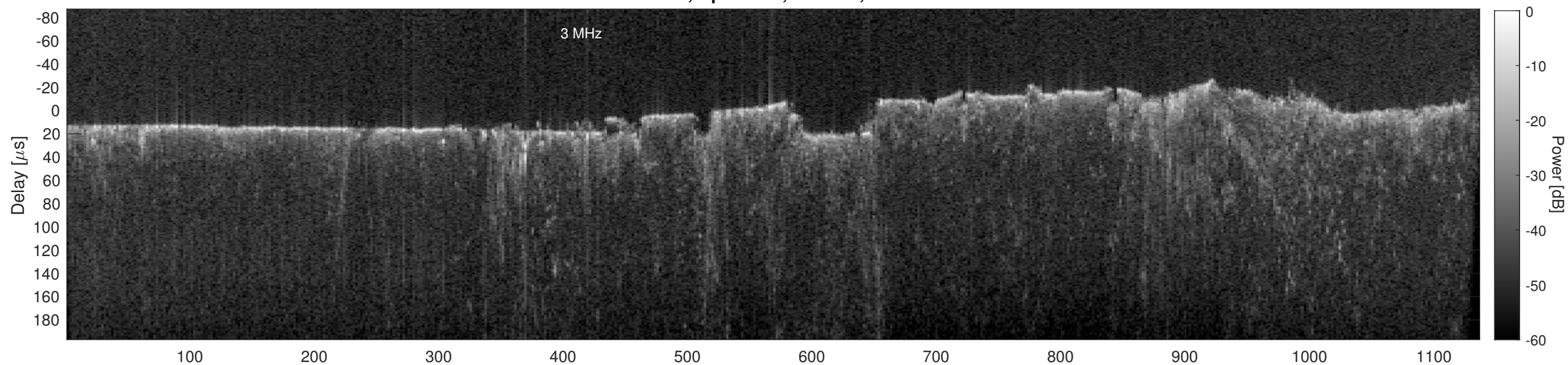
Orbit 13429, Cluttergram
