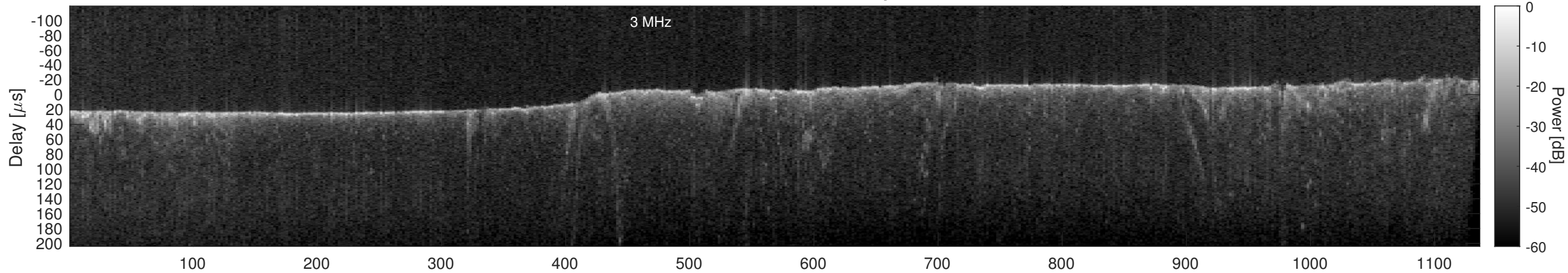
Orbit 13431, Cluttergram
