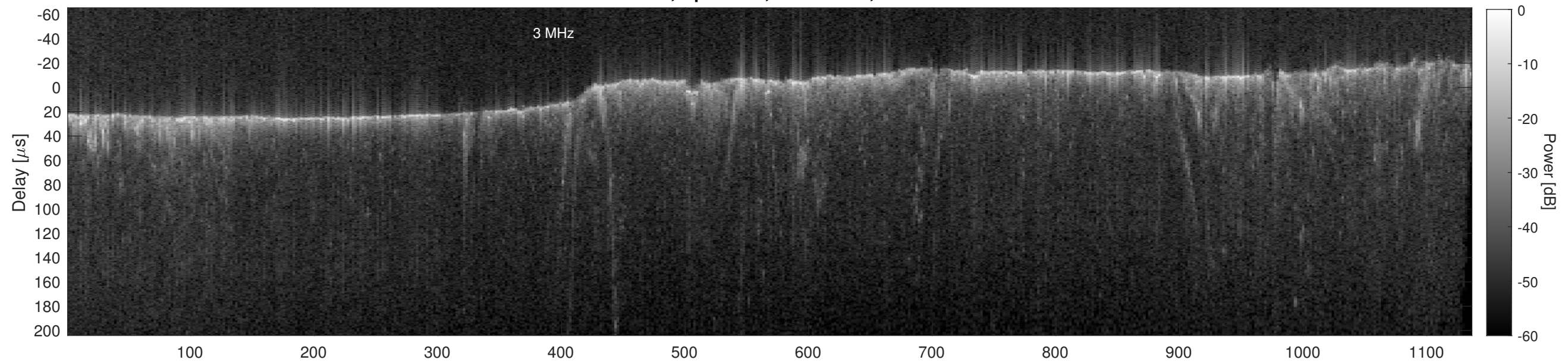
Orbit 13431, Cluttergram
