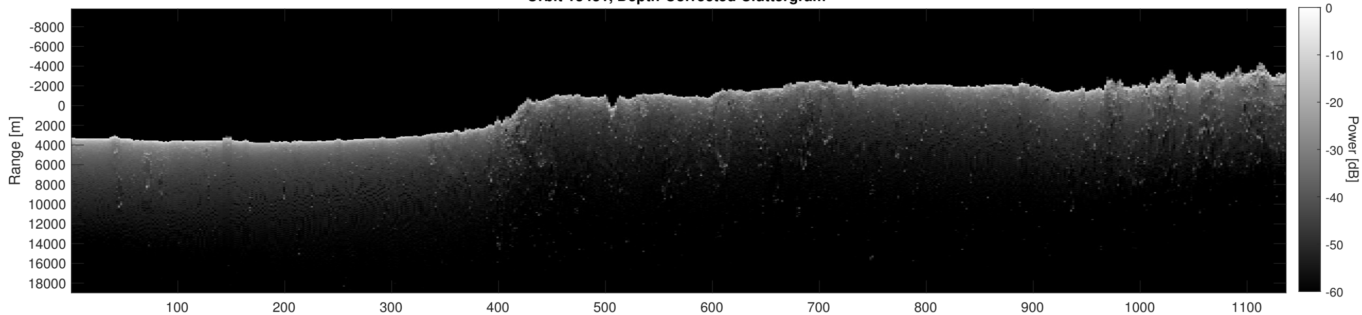
Orbit 13431, Depth-Corrected Cluttergram
