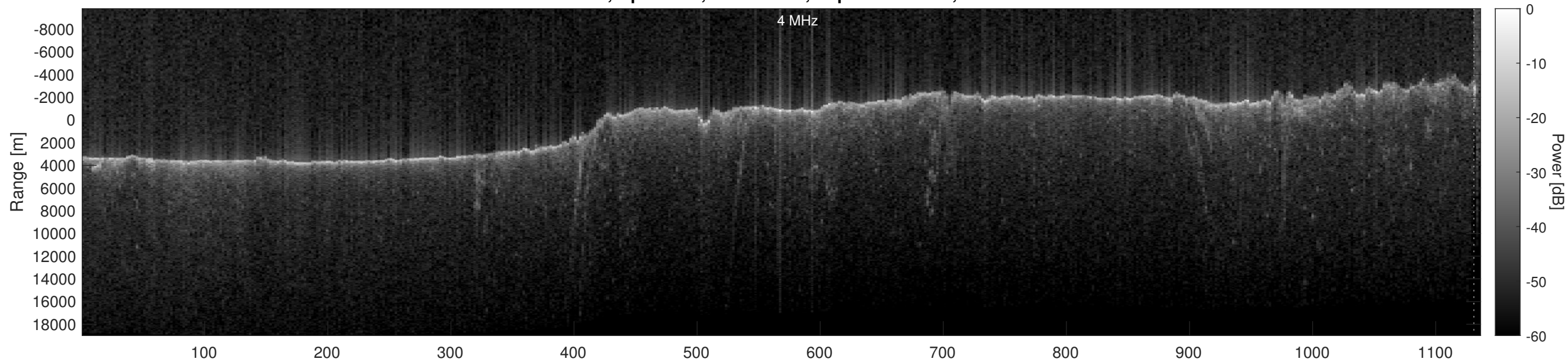
Orbit 13431, Optimized, No Window, Depth-Corrected, Channel 2
