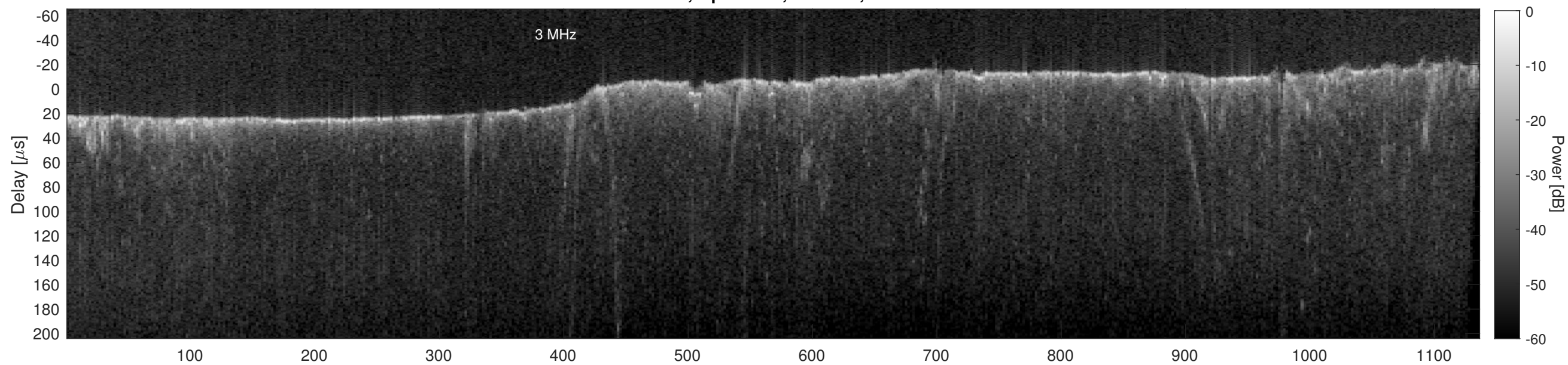
Orbit 13431, Cluttergram
