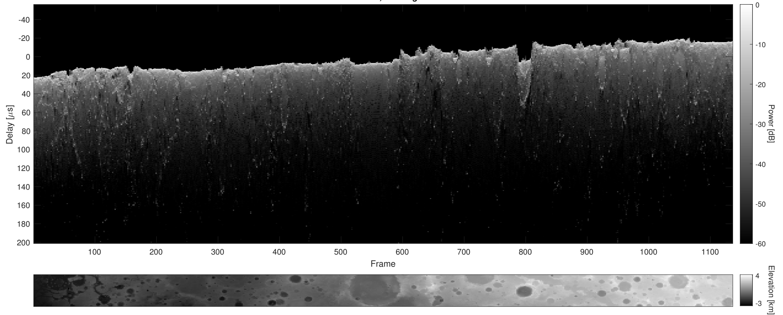
Orbit 13432, Cluttergram
