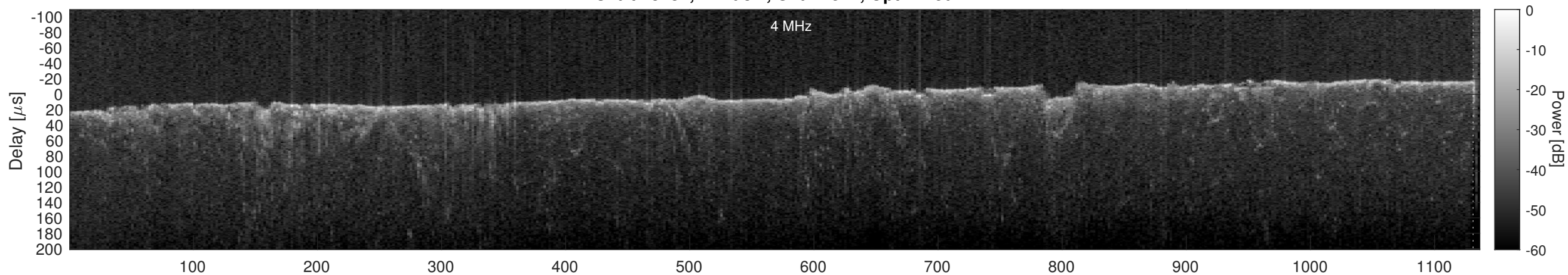
Orbit 13432, Cluttergram
