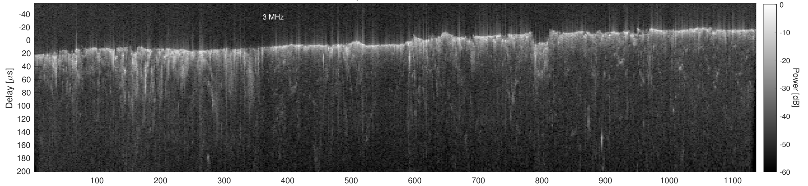
Orbit 13432, Cluttergram
