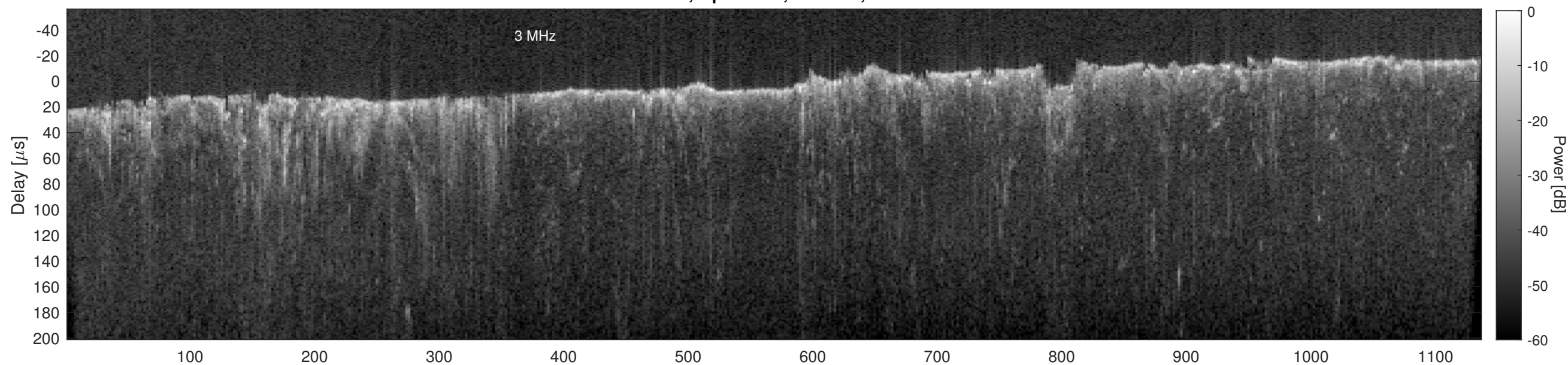
Orbit 13432, Cluttergram
