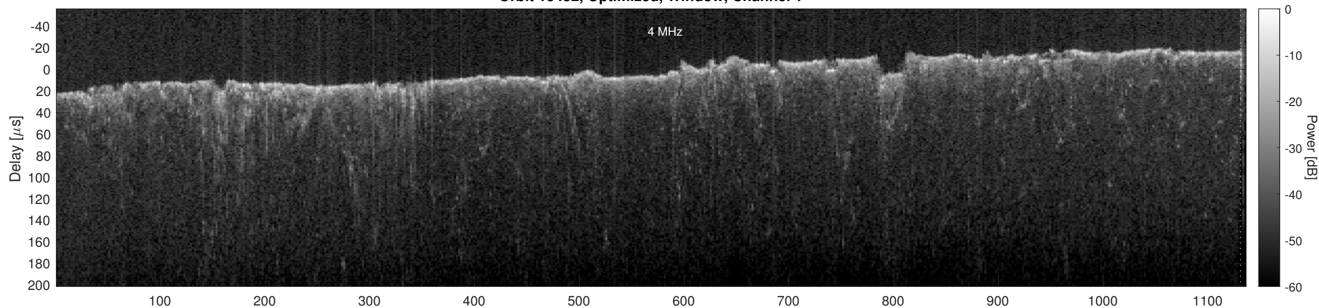
Orbit 13432, Optimized, Window, Channel 2
