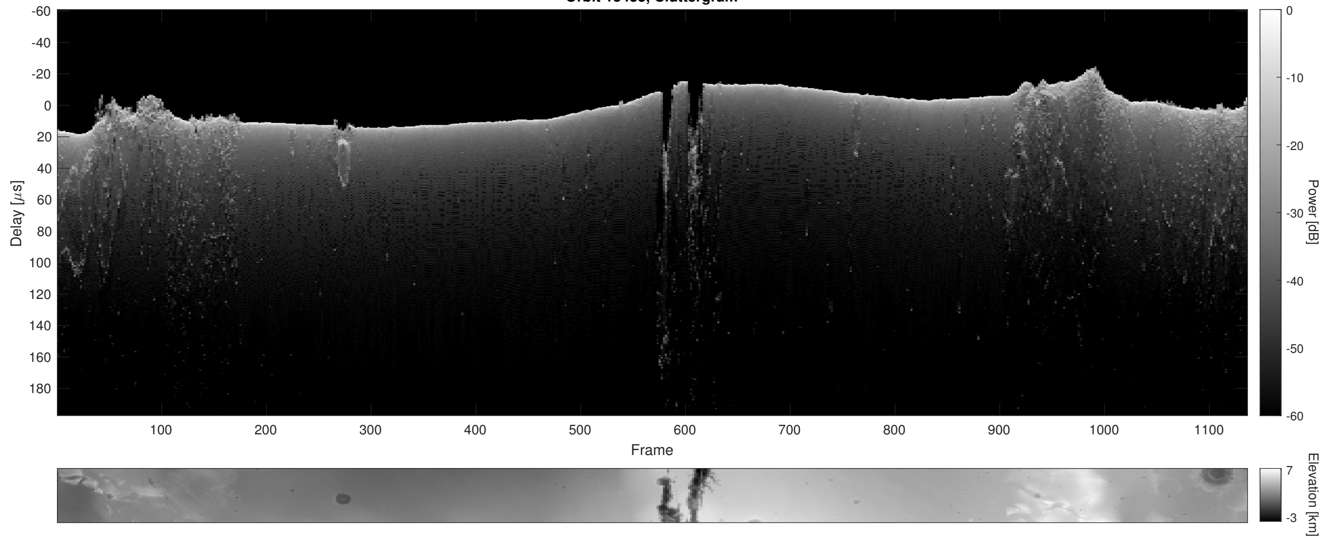
Orbit 13433, Cluttergram
