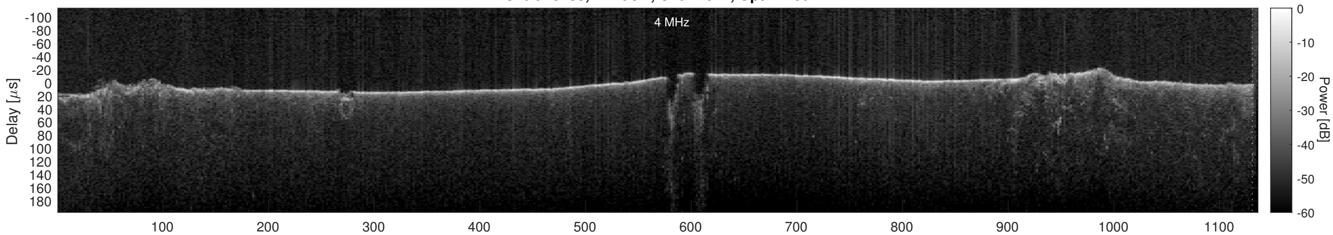
Orbit 13433, Cluttergram
