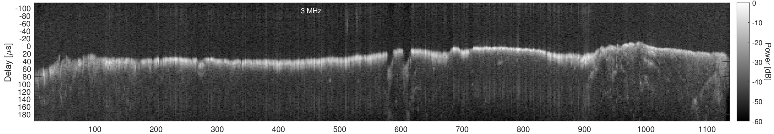
Orbit 13433, Window, Channel 2, Chapman
