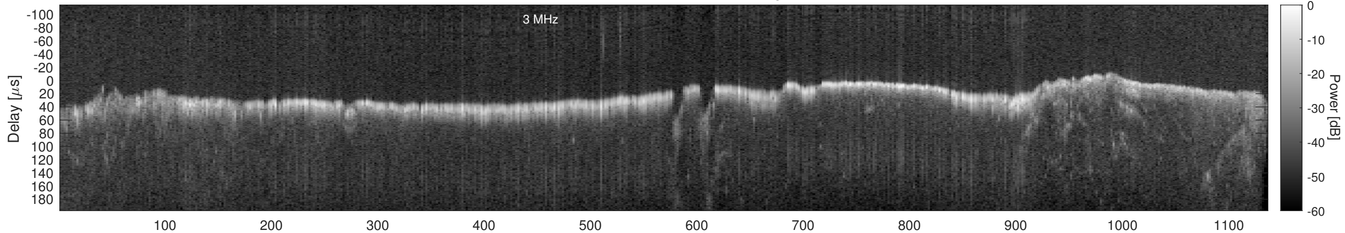
Orbit 13433, Window, Channel 2, Optimized
