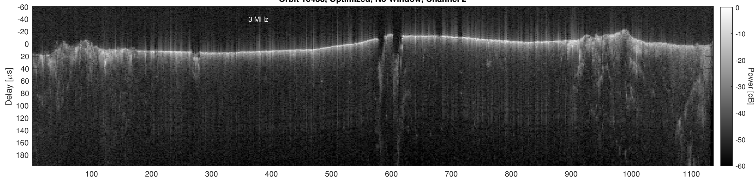
Orbit 13433, Cluttergram
