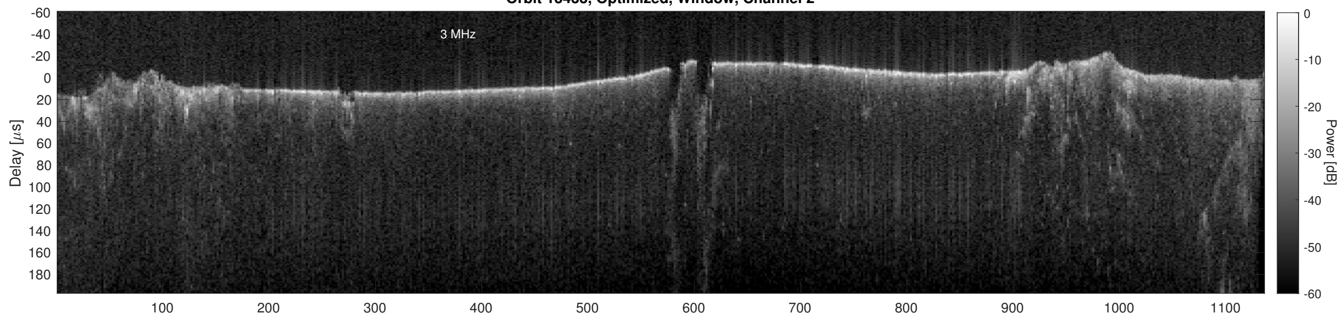
Orbit 13433, Cluttergram
