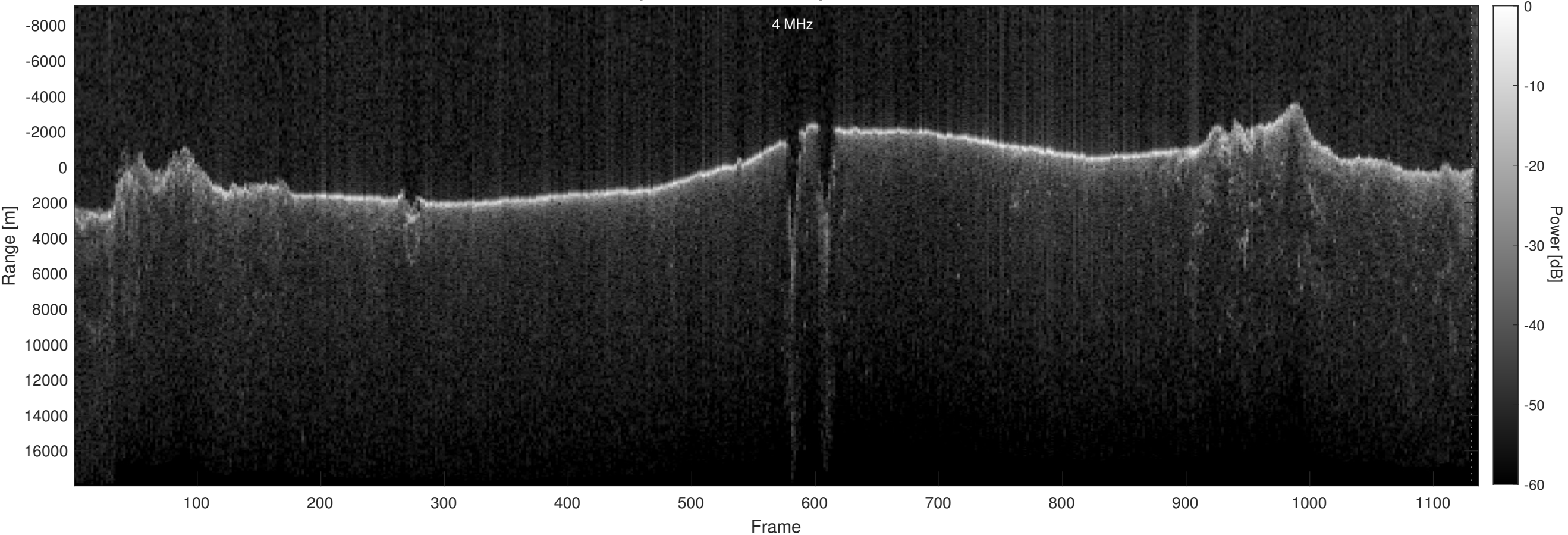
Orbit 13433, Optimized, Window, Depth-Corrected, Channel 2
