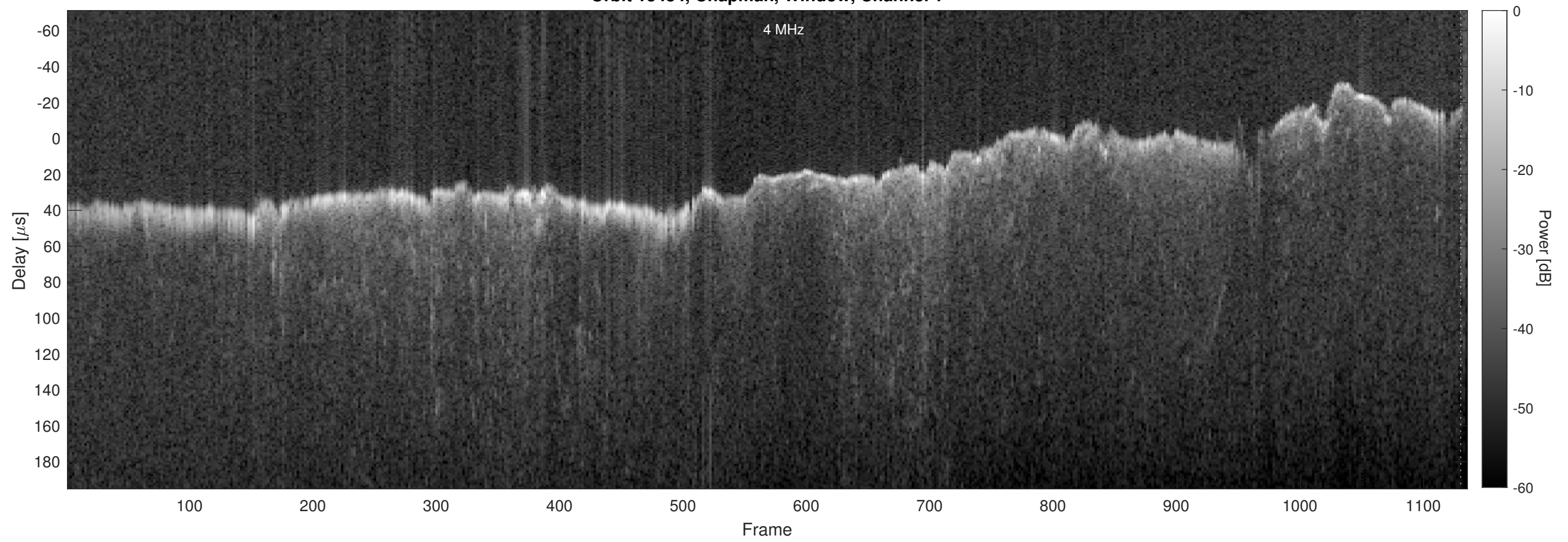
Orbit 13434, Chapman, Window, Channel 2
