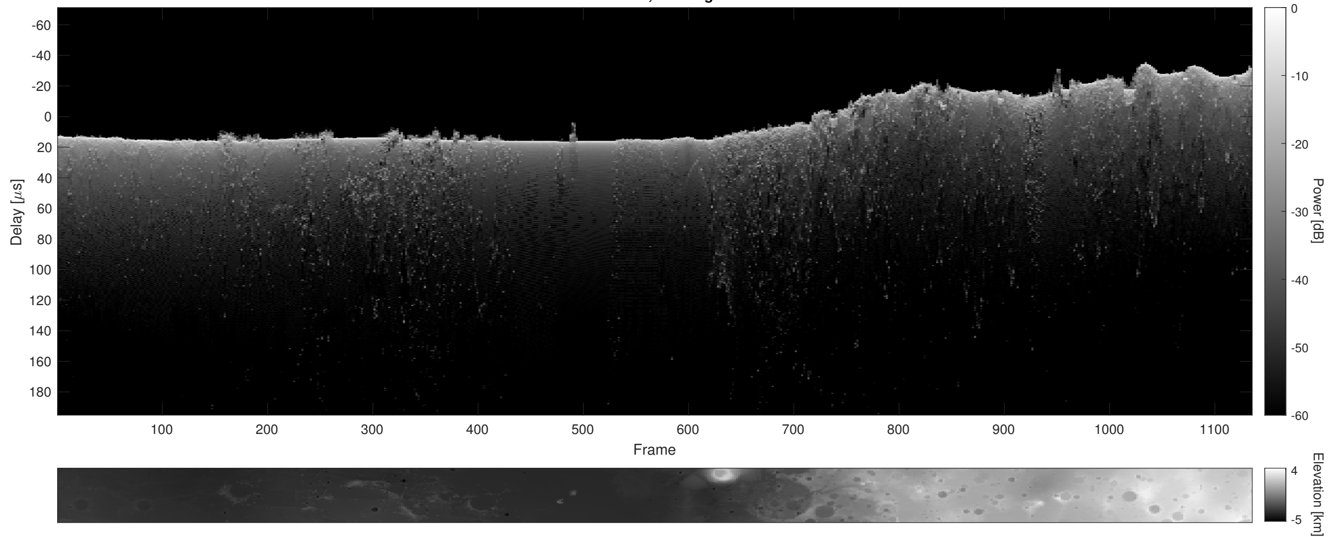
Orbit 13434, Cluttergram
