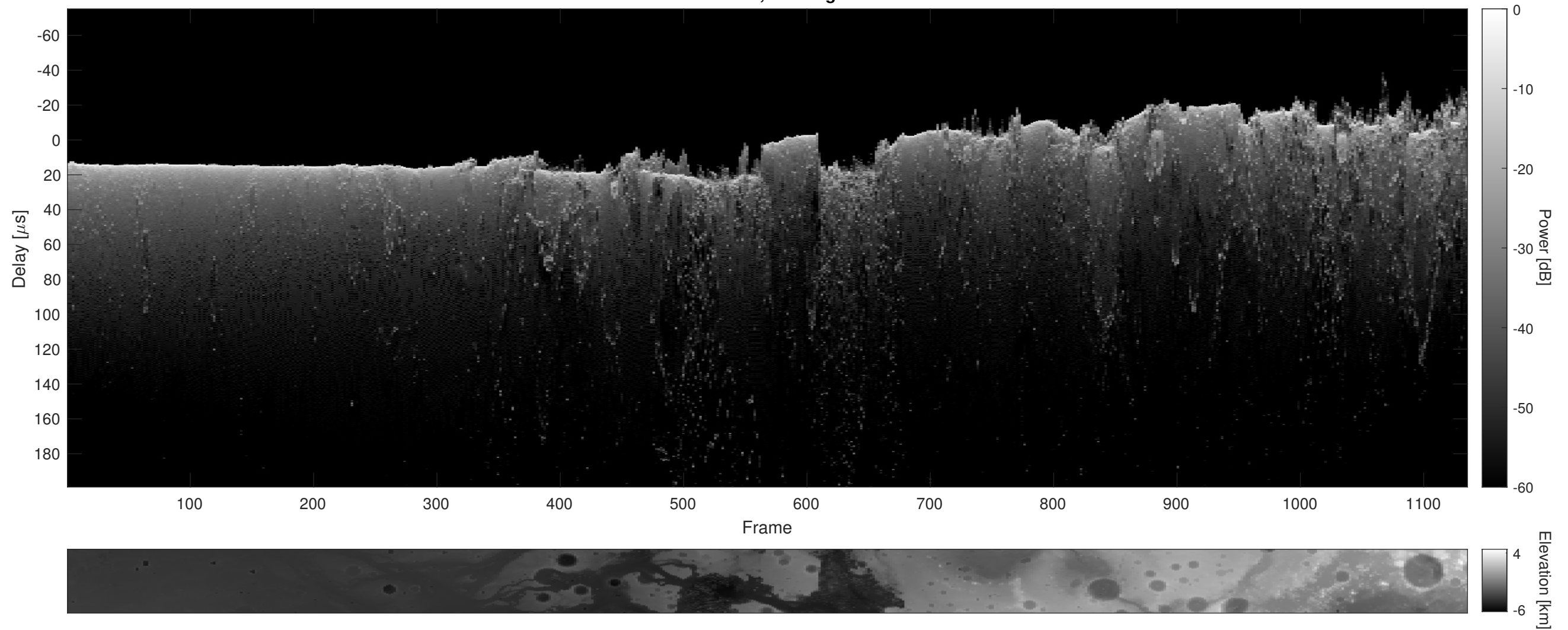
Orbit 13436, Cluttergram
