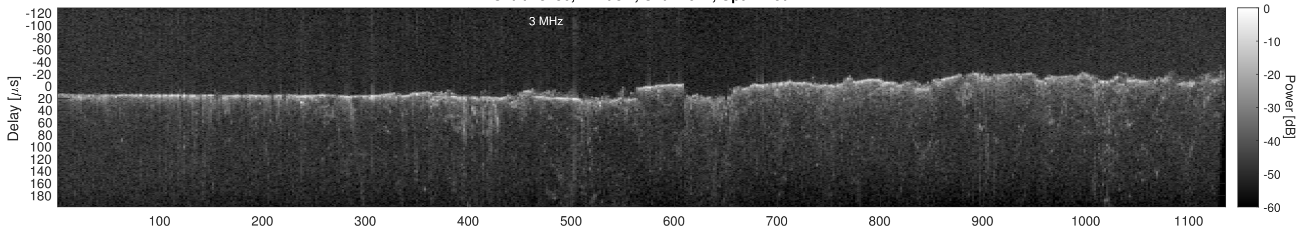
Orbit 13436, Cluttergram
