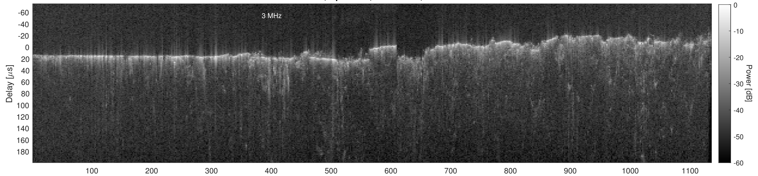
Orbit 13436, Cluttergram
