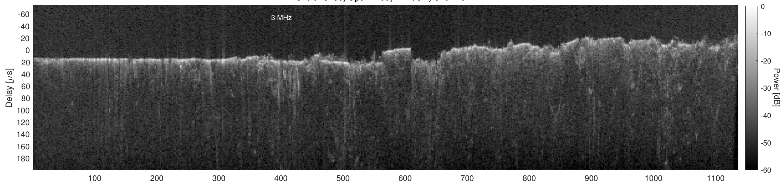
Orbit 13436, Cluttergram
