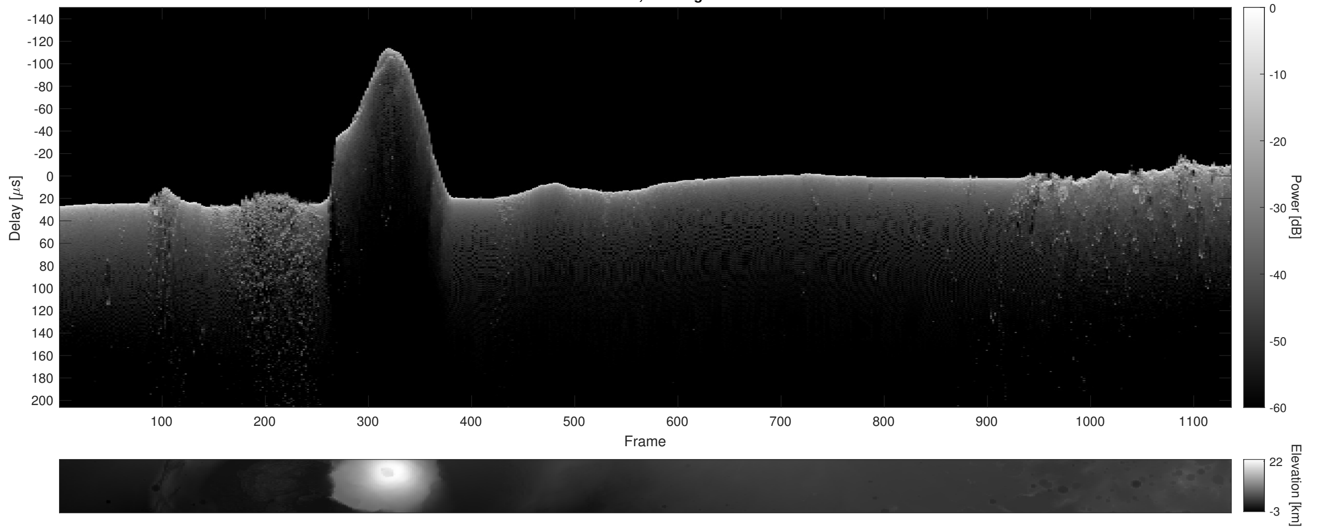
Orbit 13437, Cluttergram
