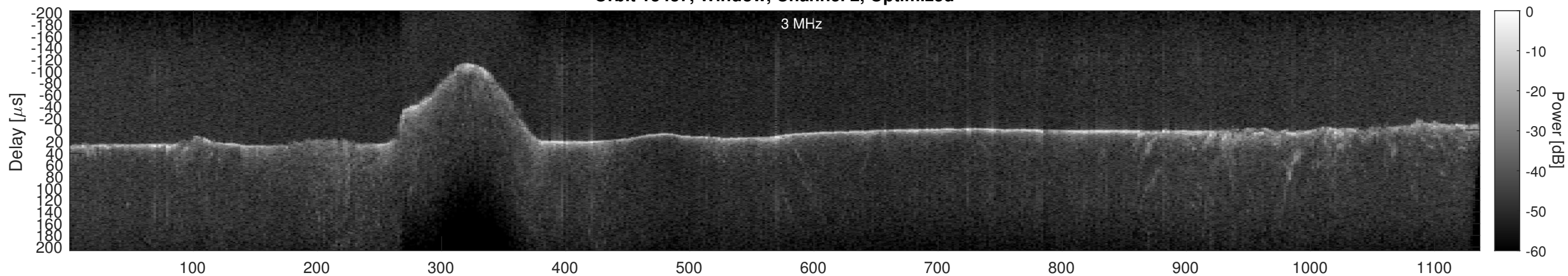
Orbit 13437, Cluttergram
