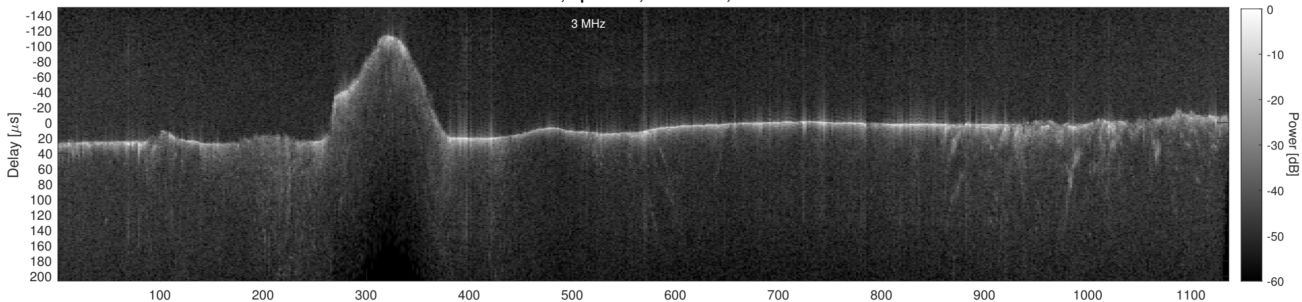
Orbit 13437, Cluttergram
