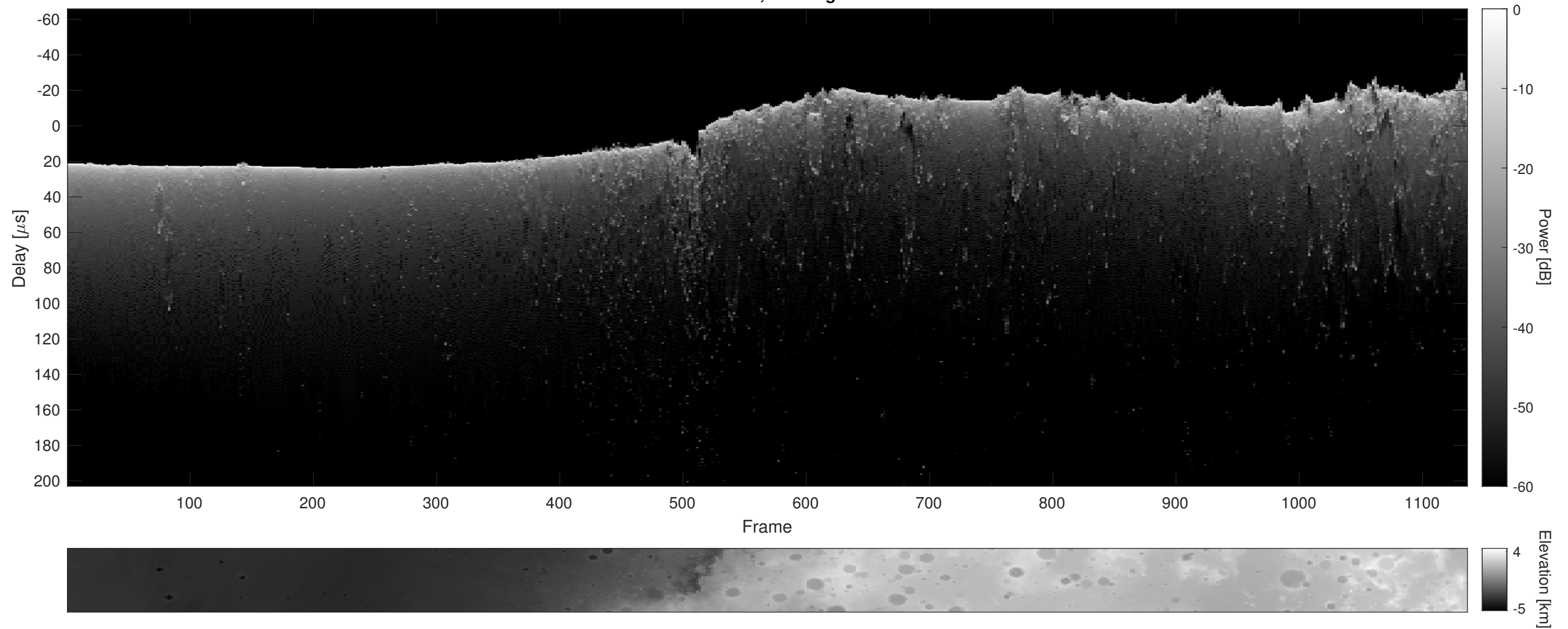
Orbit 13438, Cluttergram
