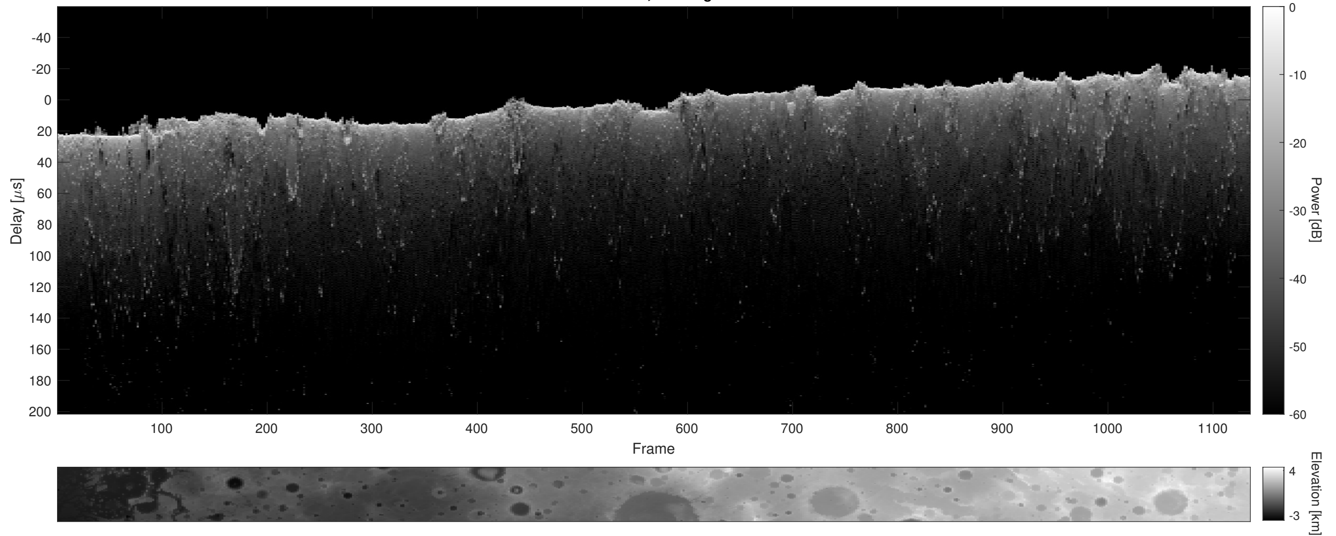
Orbit 13439, Cluttergram
