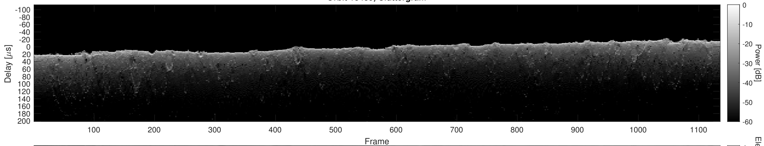
Orbit 13439, Cluttergram
