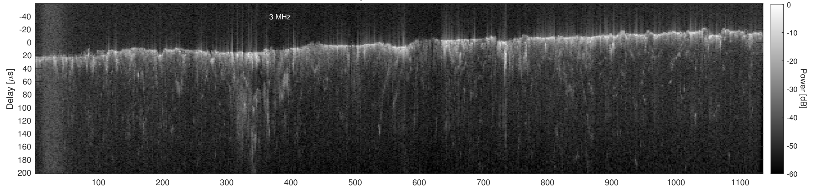
Orbit 13439, Cluttergram
