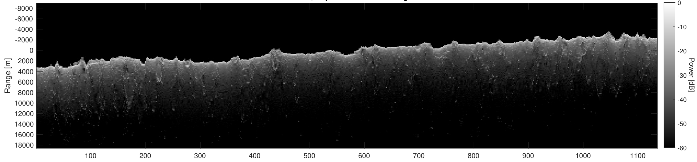
Orbit 13439, Depth-Corrected Cluttergram
