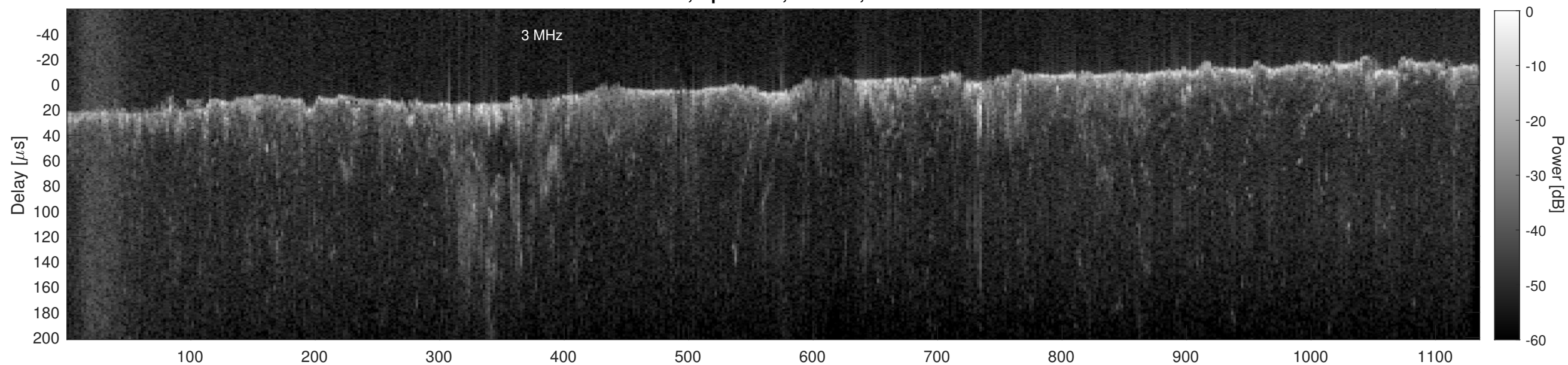
Orbit 13439, Cluttergram
