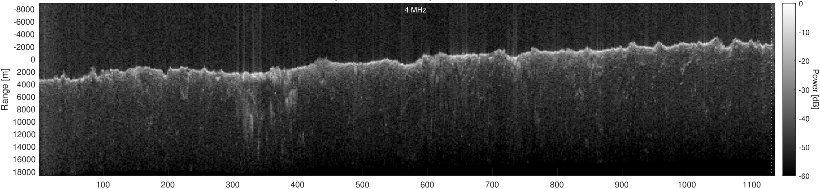
Orbit 13439, Optimized, Window, Depth-Corrected, Channel 2
