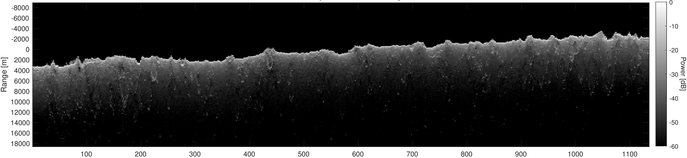
Orbit 13439, Depth-Corrected Cluttergram
