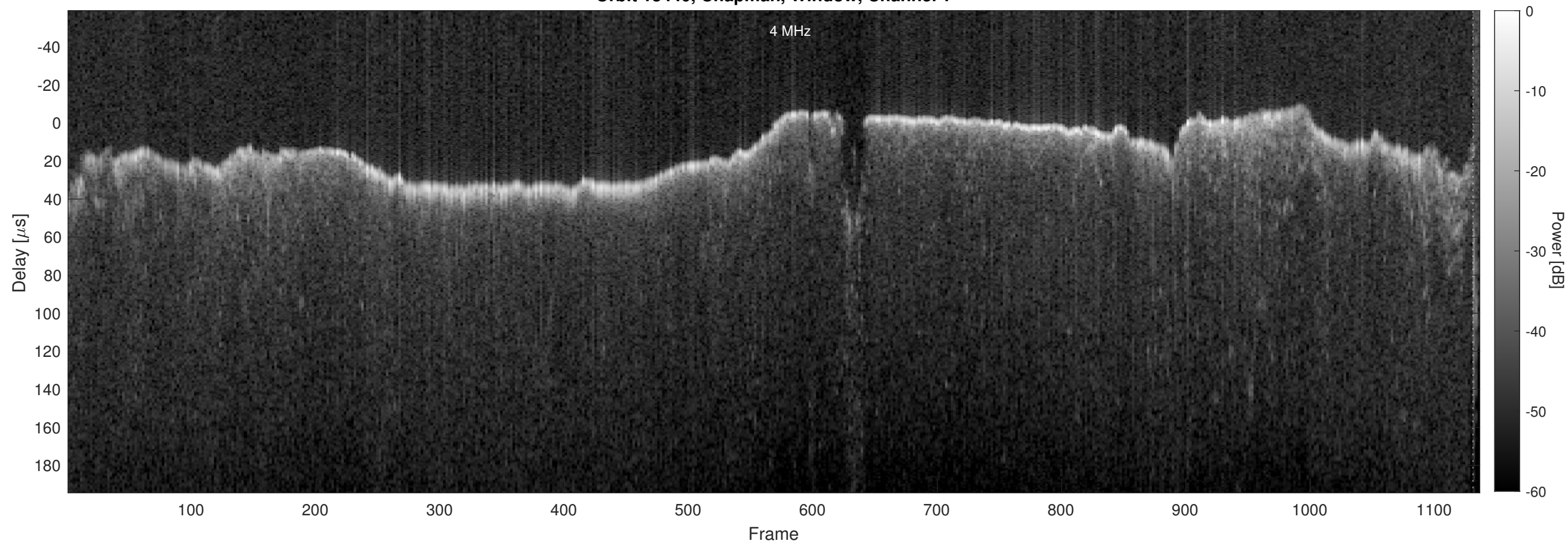
Orbit 13440, Chapman, Window, Channel 2
