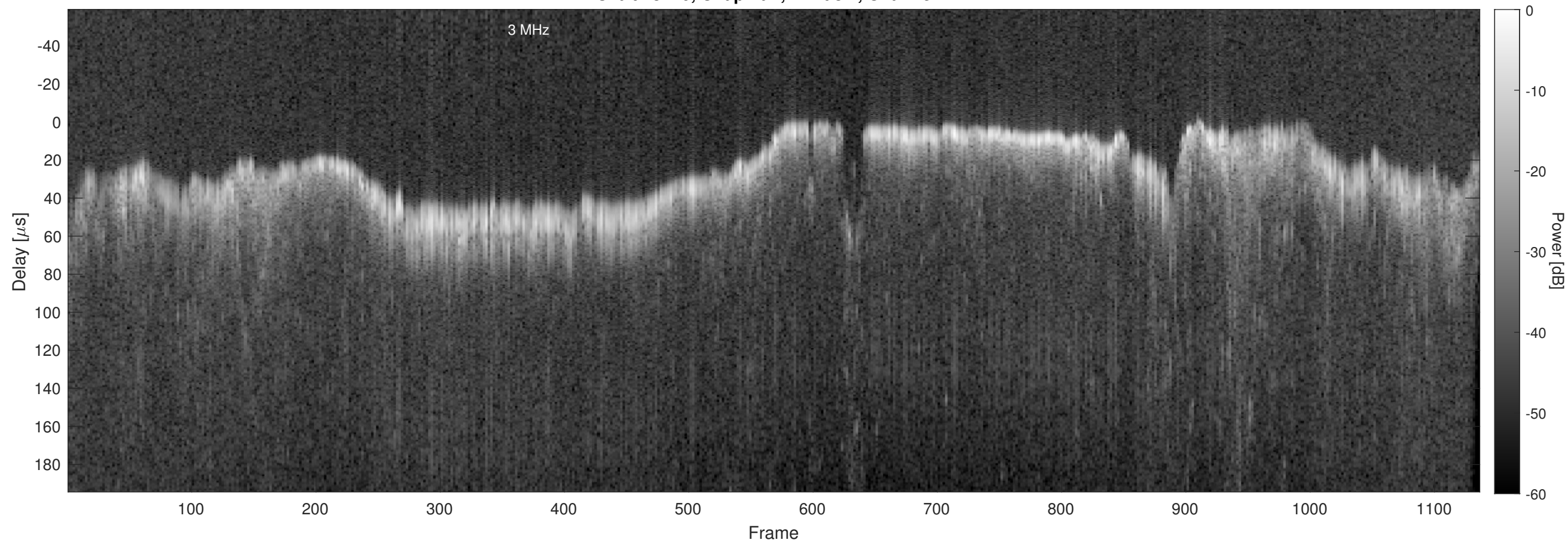
Orbit 13440, Chapman, Window, Channel 2
