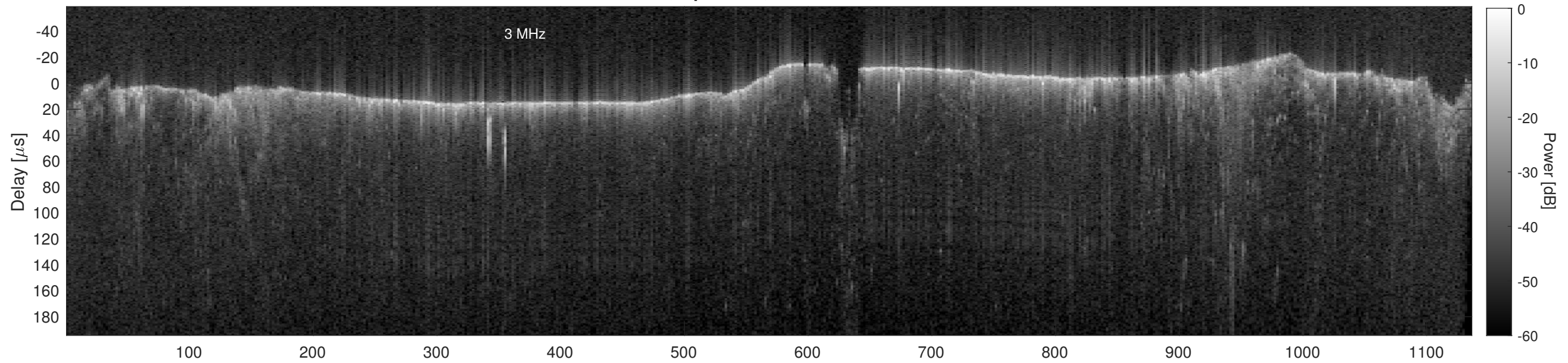
Orbit 13440, Cluttergram
