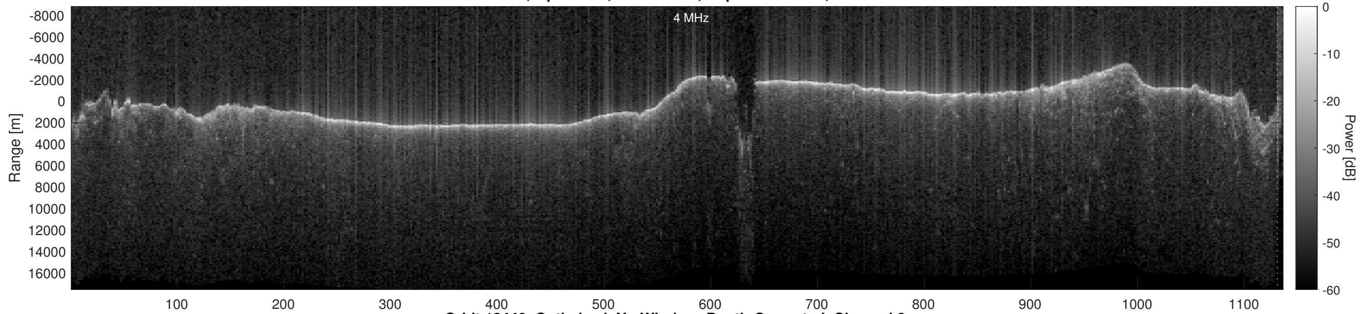
Orbit 13440, Optimized, No Window, Depth-Corrected, Channel 2
