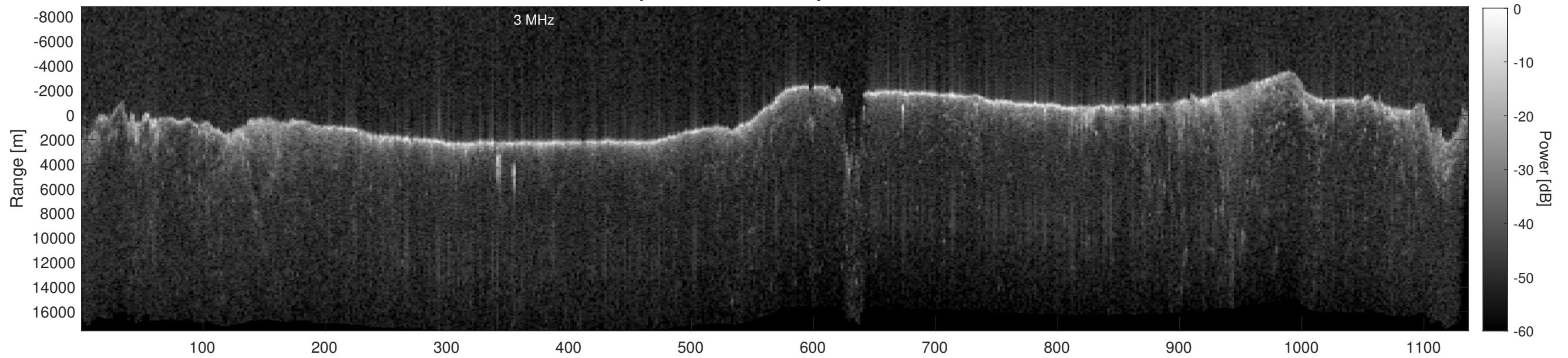
Orbit 13440, Depth-Corrected Cluttergram
