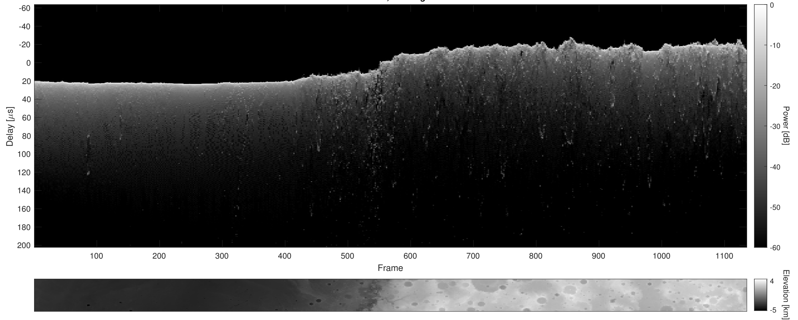
Orbit 13445, Cluttergram
