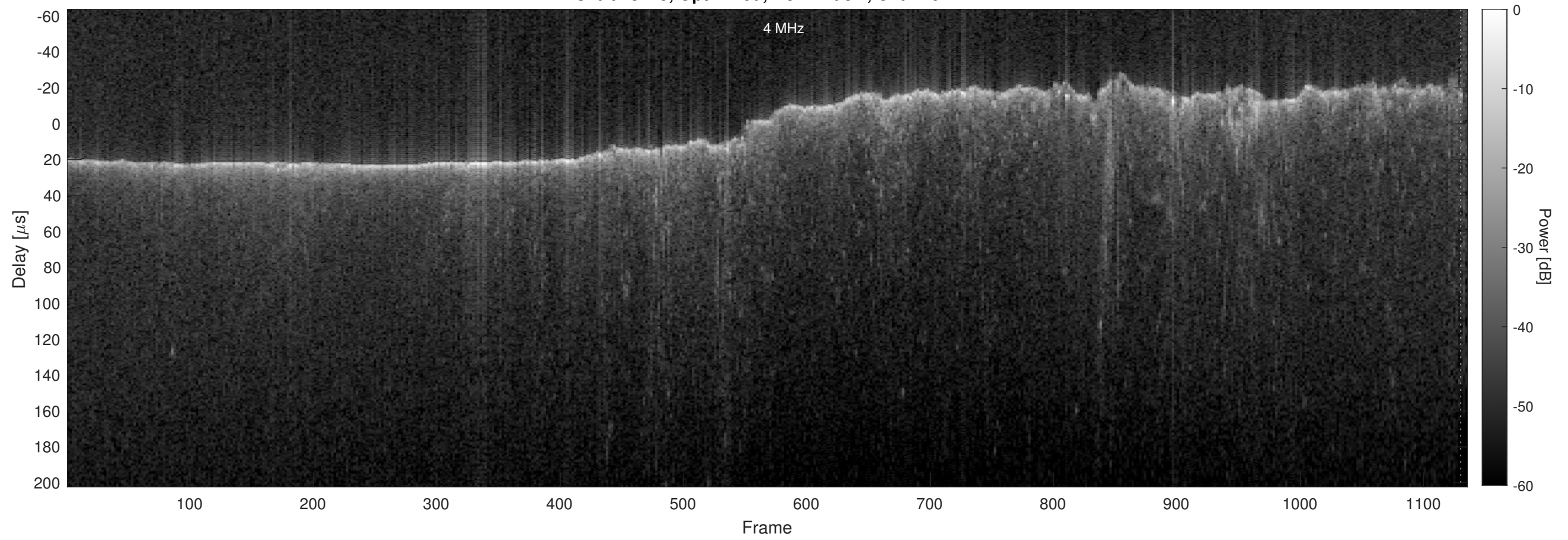
Orbit 13445, Optimized, No Window, Channel 2
