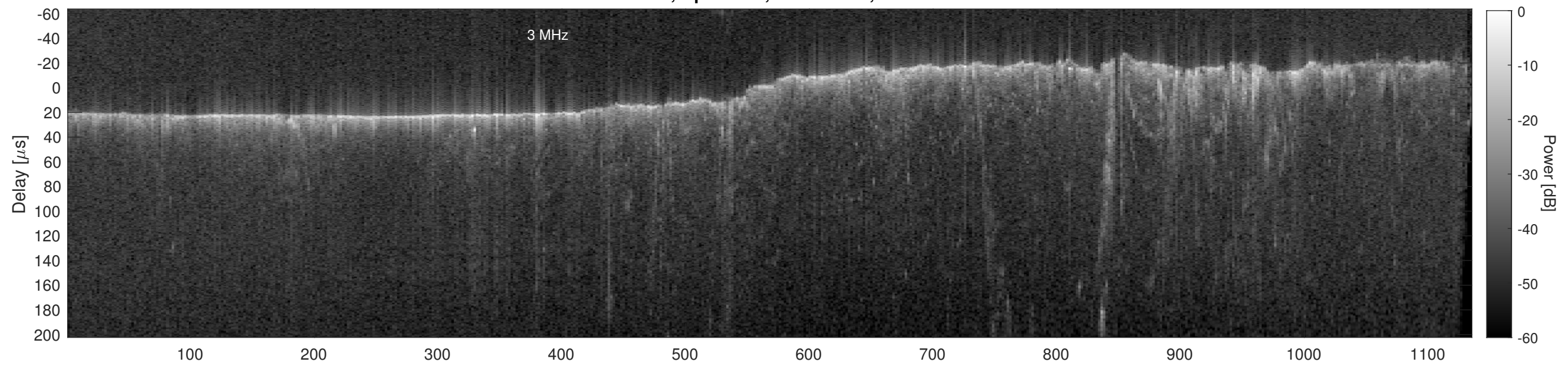
Orbit 13445, Cluttergram
