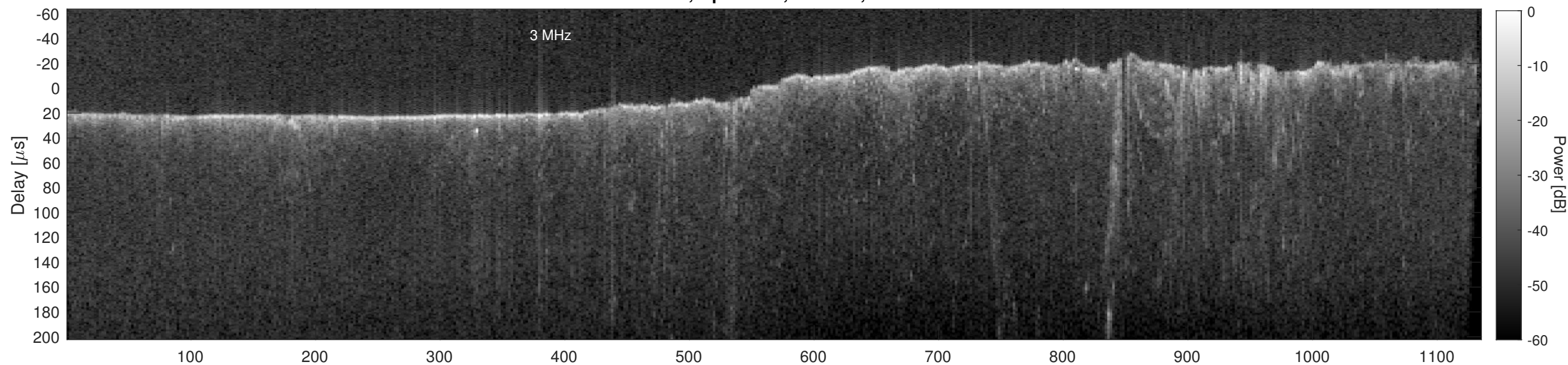
Orbit 13445, Cluttergram
