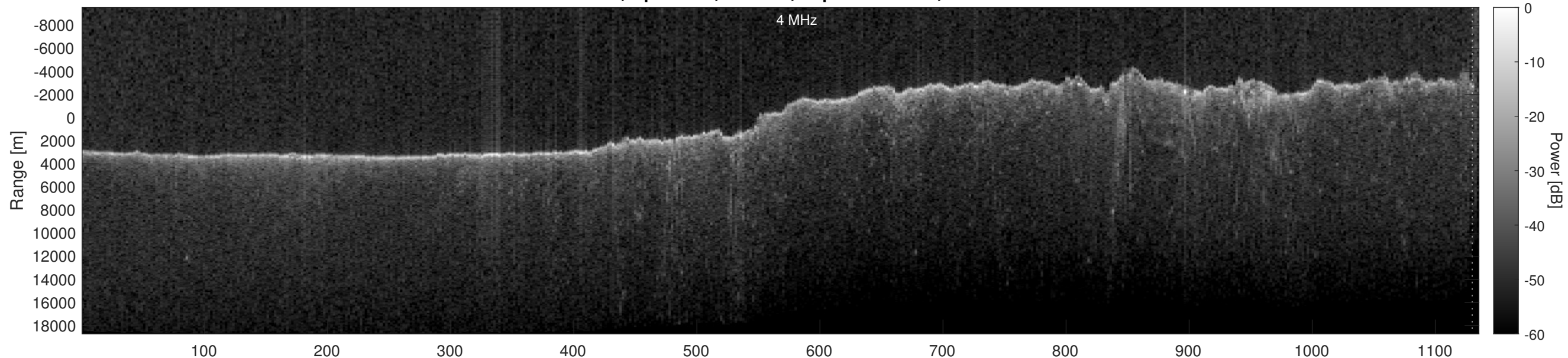
Orbit 13445, Optimized, Window, Depth-Corrected, Channel 2
