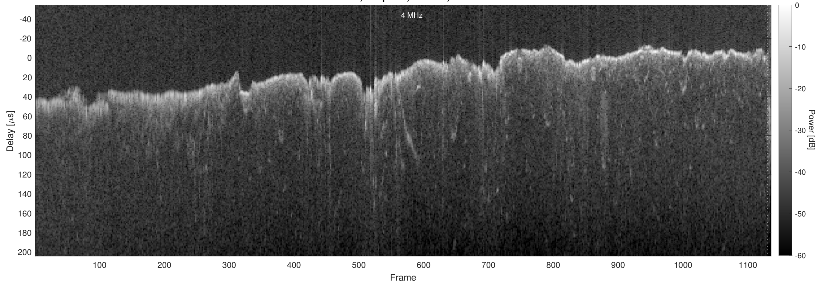
Orbit 13446, Chapman, Window, Channel 2
