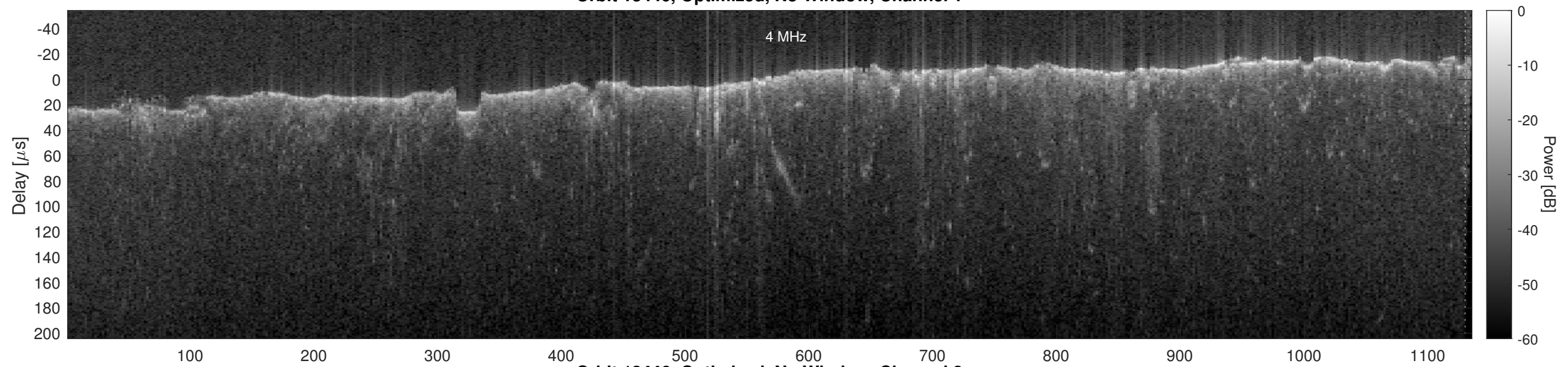
Orbit 13446, Optimized, No Window, Channel 2
