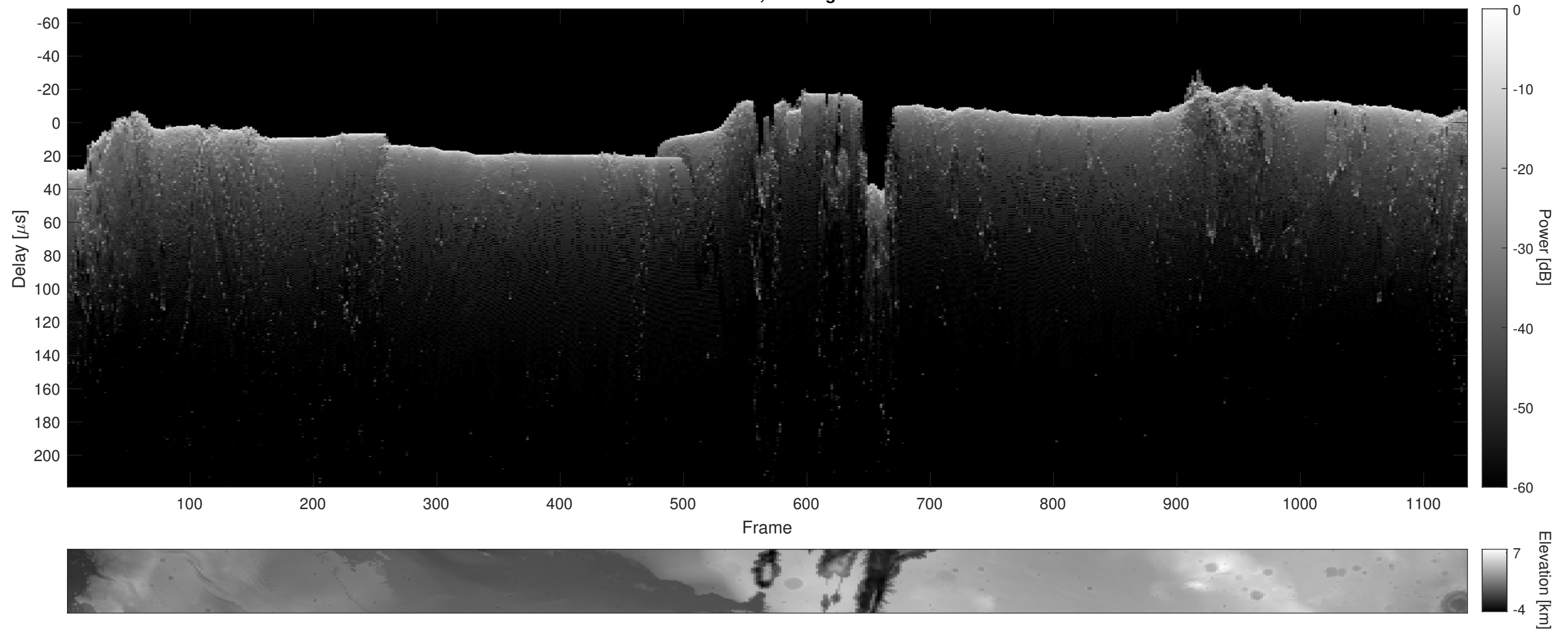
Orbit 13447, Cluttergram
